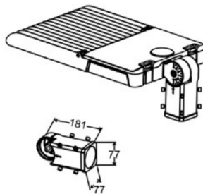
Bracket C
